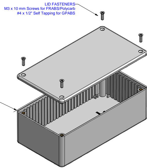
EXPLODED VIEW OF ENCLOSURE
